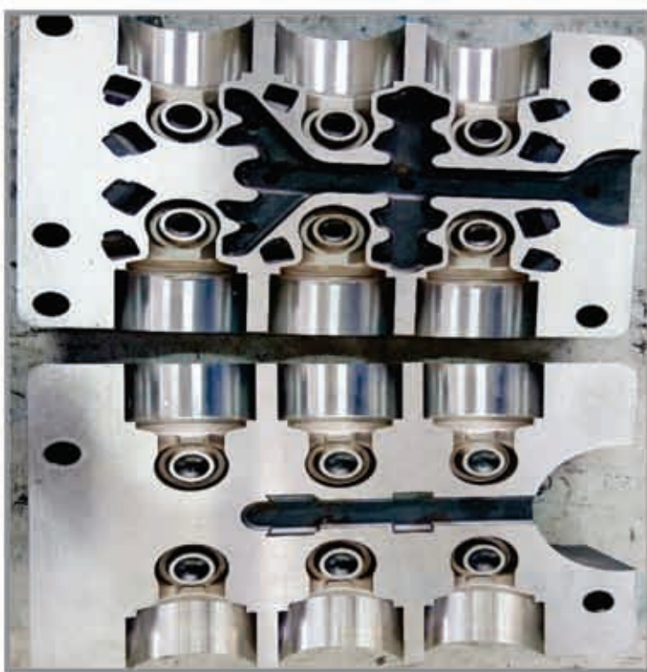
Development of tool for automotive component manufacturing
